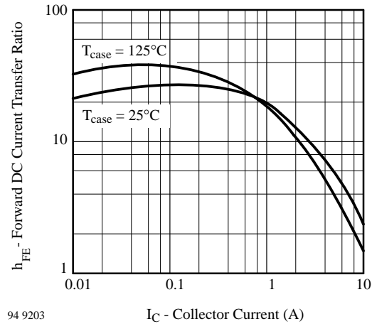
Figure 8. h_{FE} vs. I_C
